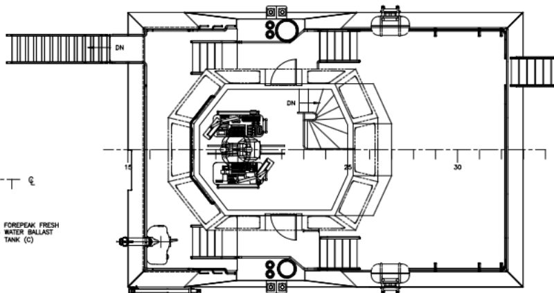
BRIDGE DECK PLAN
