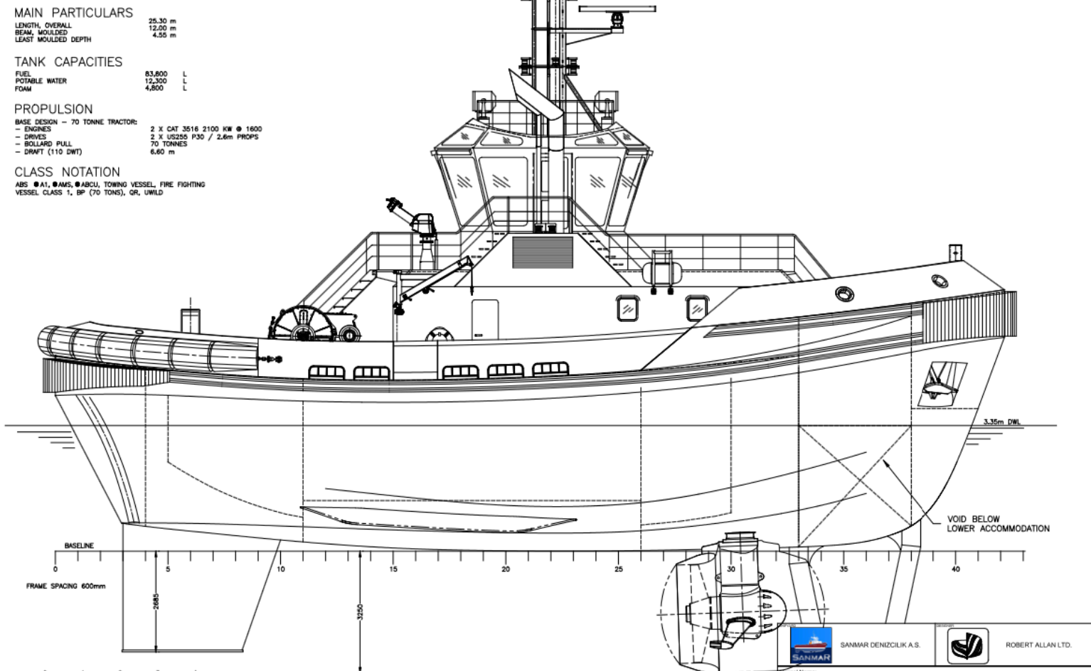
OUTBOARD PROFILE
