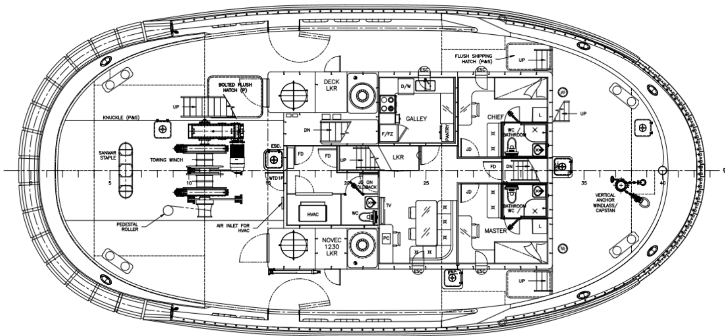
MAIN DECK PLAN
