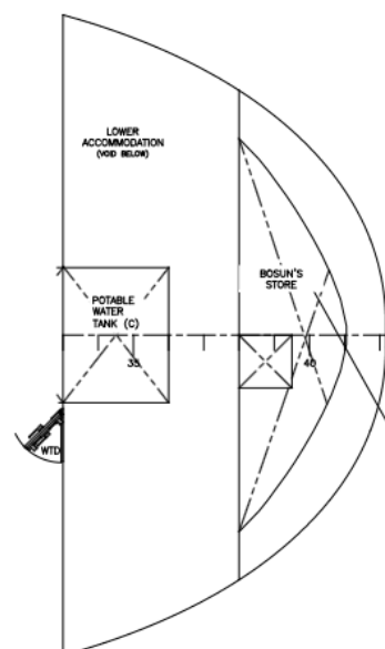
VOID BELOW ACCOMMODATION
