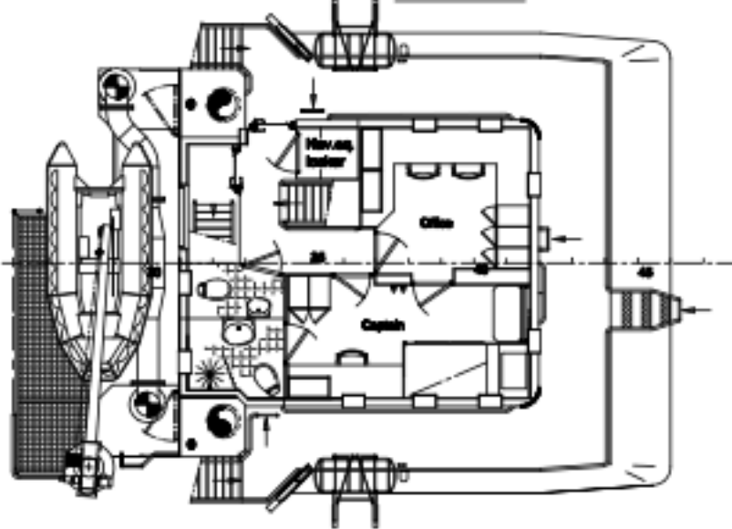
Boatdeck
