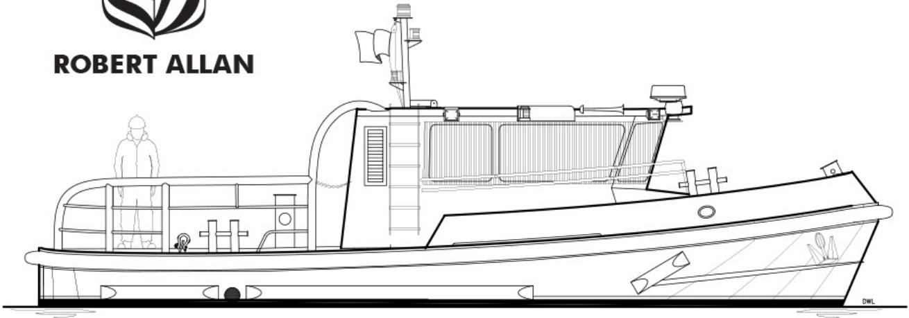
OUTBOARD PROFILE
