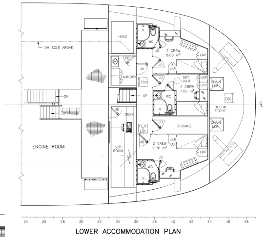
LOWER ACCOMMODATION PLAN
