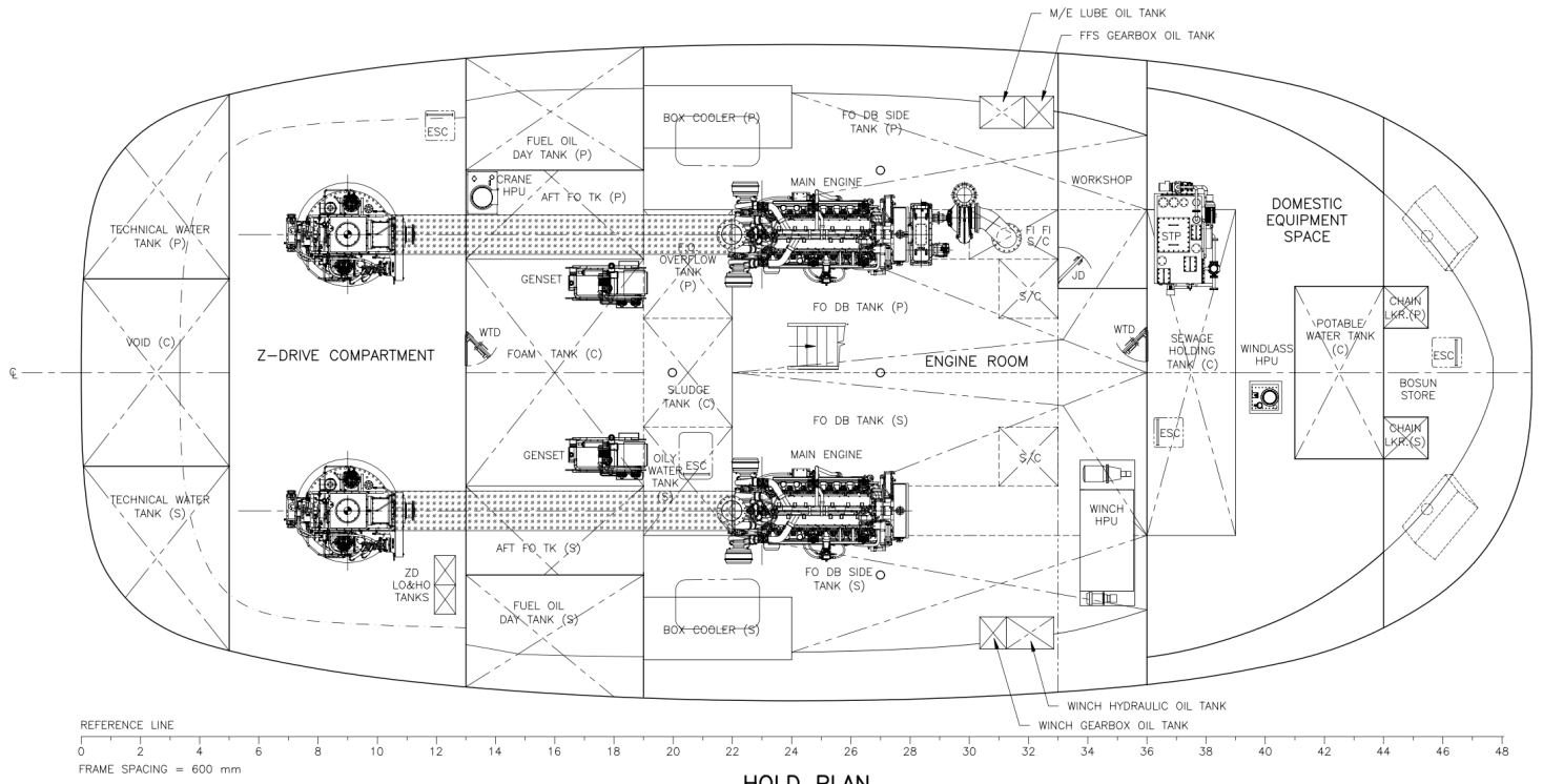
HOLD PLAN
